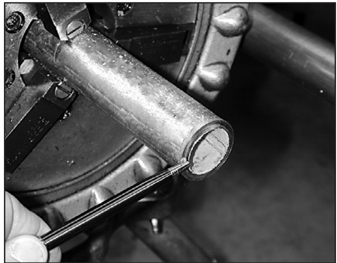
Figure 6: The roll cutter will leave a burr on the inside diameter of the conduit. The burr must be removed to ensure that the wire insulation will not be damaged during pulling.
