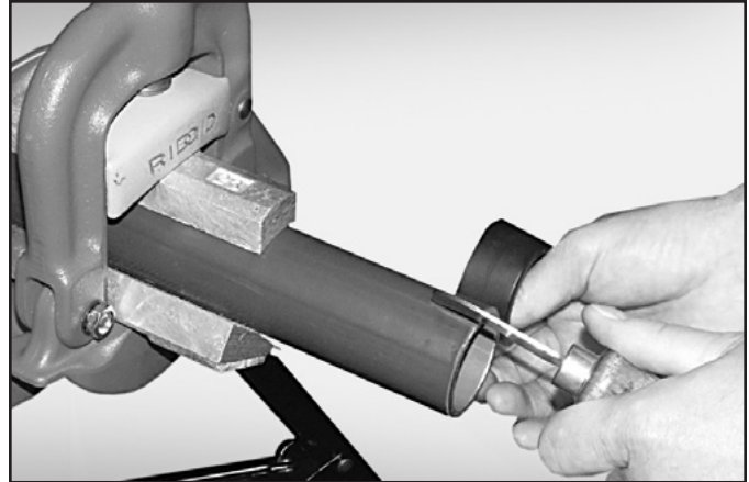
Figure 17: Before threading PVC-coated conduit , make a series of cuts along the axis of the conduit to break-up threading chip.
