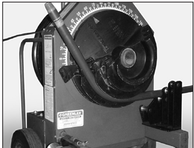
Figure 19: Bender with special shoes required for bending PVC-coated conduit.
