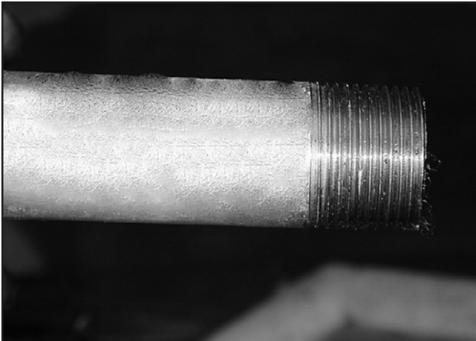
Figure 12: A proper thread should be free from chips or tears over the entire length.
